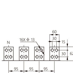
Horizontal Short Busbar (specially made)
