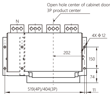
A Installation size
