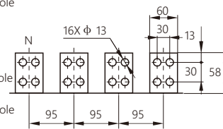
Horizontal long busbar (specially made)
