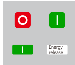
Circuit breaker switched on and no energy storage
