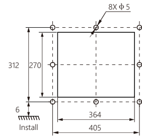
Cutout size of cabinet door
