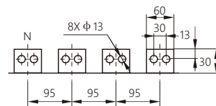
Horizontal Short Busbar (Default Configuration)
