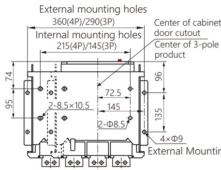
A-direction mounting dimensions
