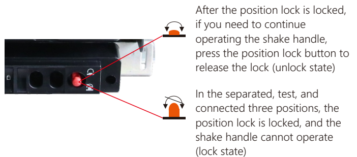
Connected position: Both the main circuit and the auxiliary circuit are connected.
