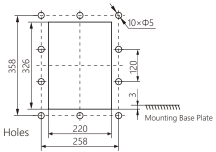
Cabinet Door Cutout Dimensions
