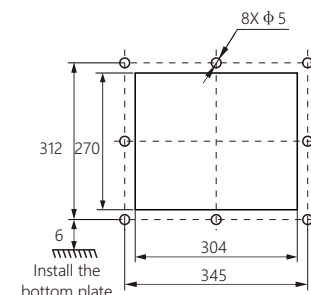
Cutout size of cabinet door
